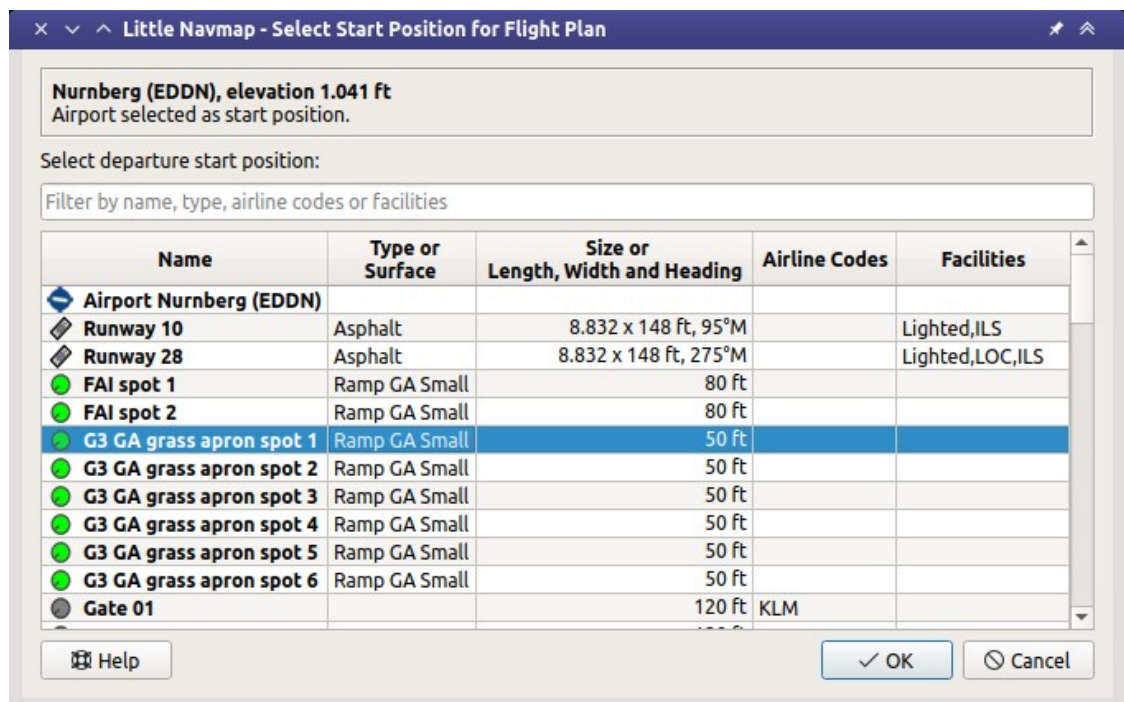
The start position selection dialog for EDDN.
