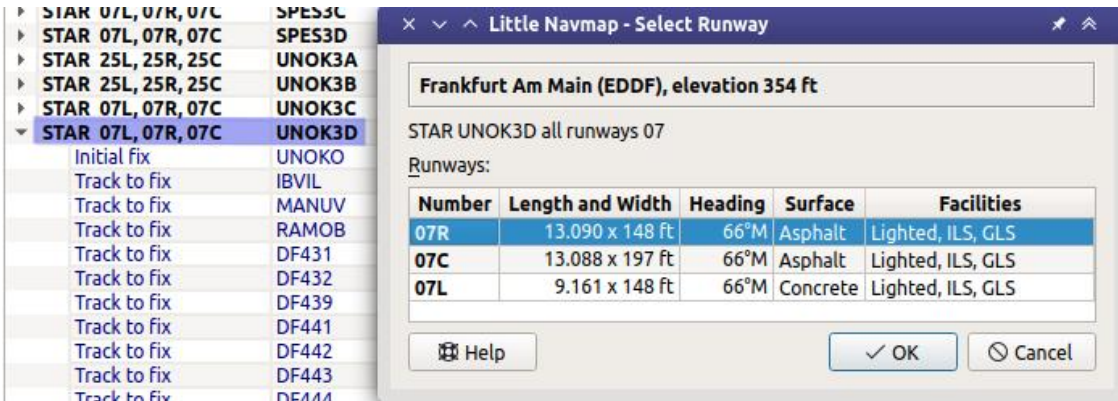
Runway selection dialog after choosing the STAR UNOK3D which applies to the three parallel runways 07R, 07C, and 07L.
