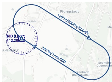
Holding at VORDME RID. Inbound label shows inbound magnetic course, holding time and navaid ident. Outbound track has outbound magnetic course, speed and altitude as label. While filled triangle is the hotspot and holding fix. Click image to enlarge.
